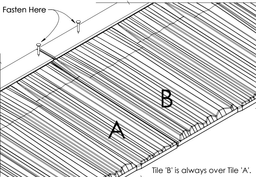
Figure 11.3 Overlap Detail
