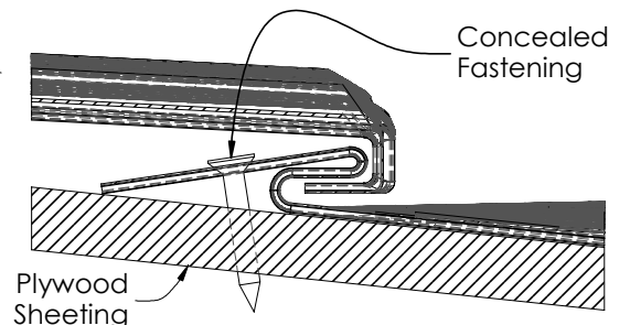
Figure 11.5 Nose Lap Detail
