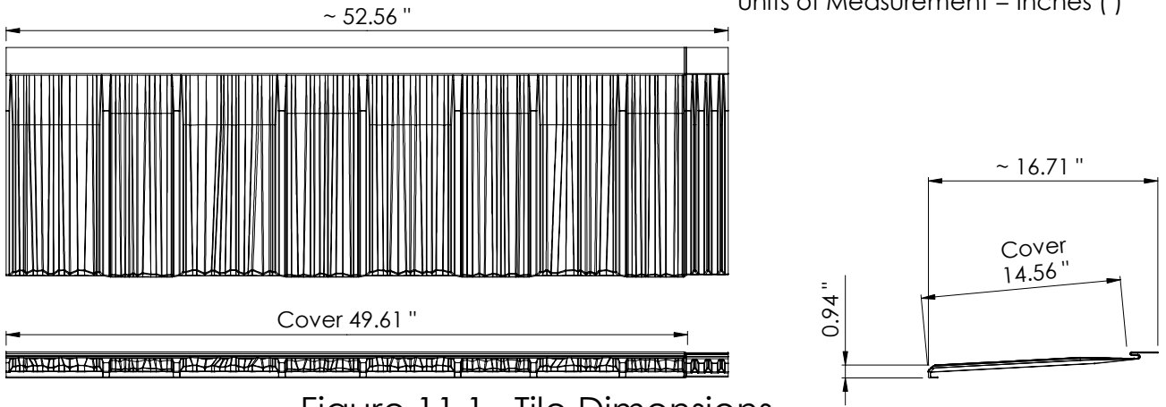
Figure 11.1 Tile Dimensions
