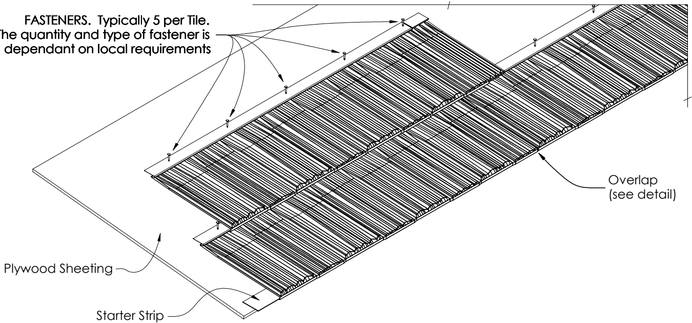
Figure 11.2 Fastening Detail
