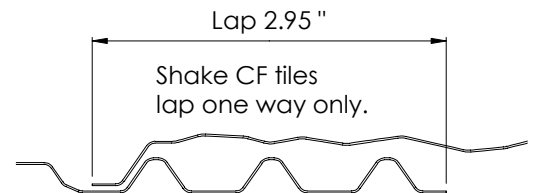
Figure 11.4 Side Lap Detail
