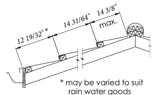
Figure 8.5 Batten Layout
