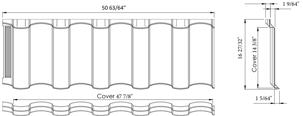
Figure 8.1 Tile Dimensions
