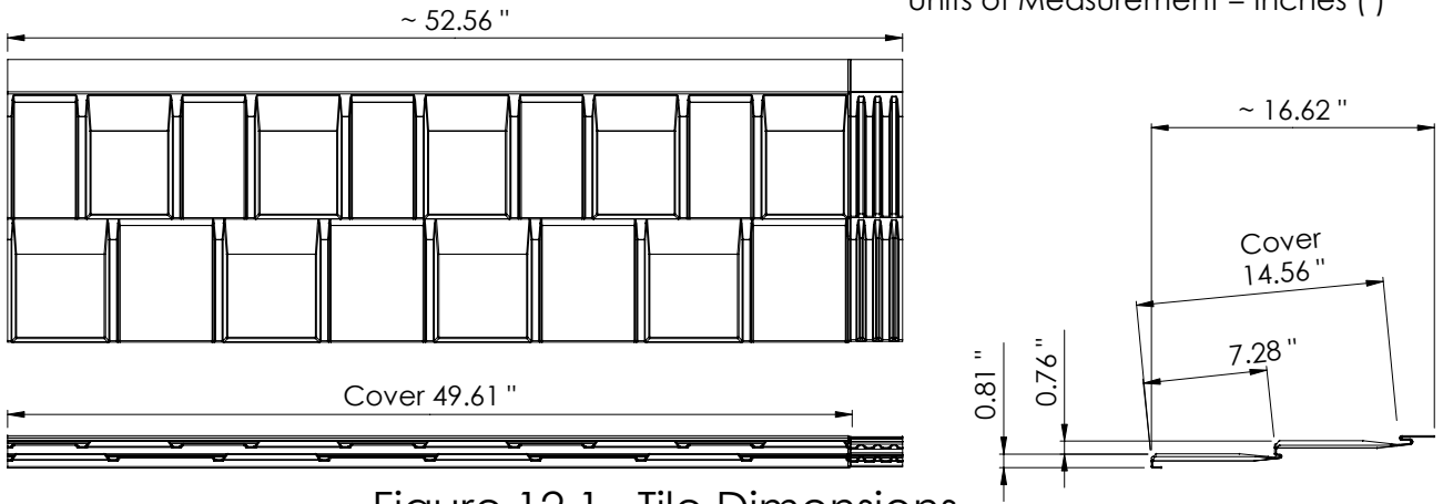
Figure 12.1 Tile Dimensions
