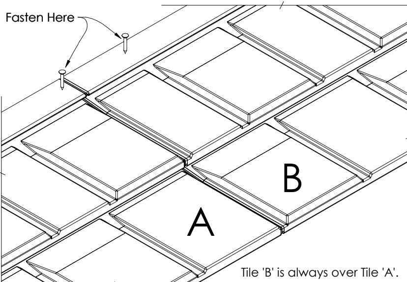
Figure 12.3 Overlap Detail
