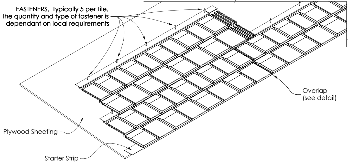
Figure 12.2 Fastening Detail
