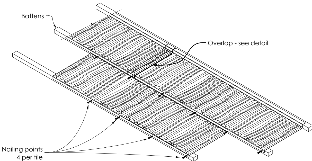
Figure 2.2 Nailing Detail
