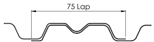
Figure 2.4 Lap Section
