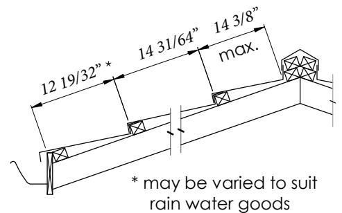
Figure 2.5 Batten Layout
