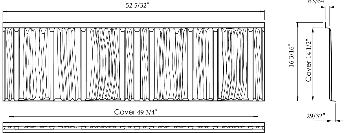
Figure 2.1 Tile Dimensions
