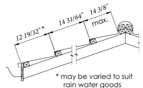
Figure 8.5 Batten Layout
