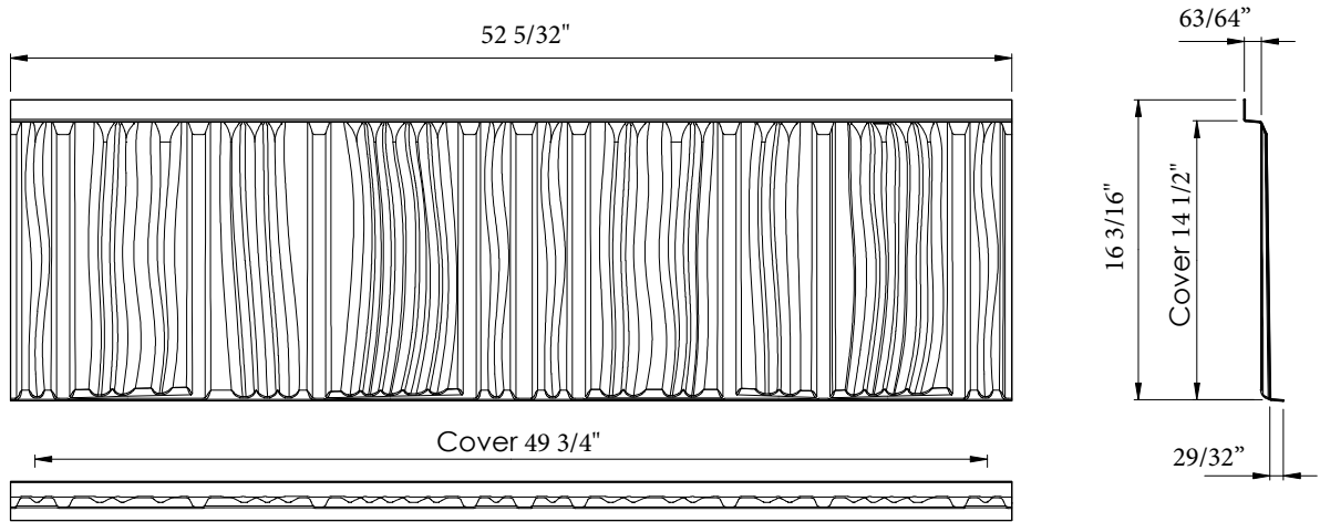
Figure 2.1 Tile Dimensions
